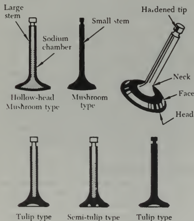
FIGURE 1-16. Valve types.
